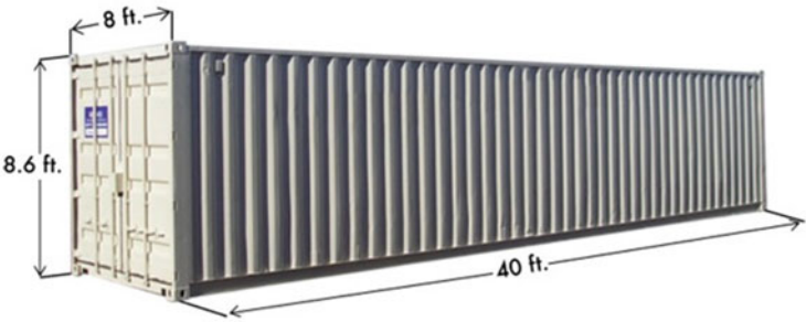
Fig. 11.1 Dimension of standard 40 ft container. (Source: Edidiwan.blogspot.com )
