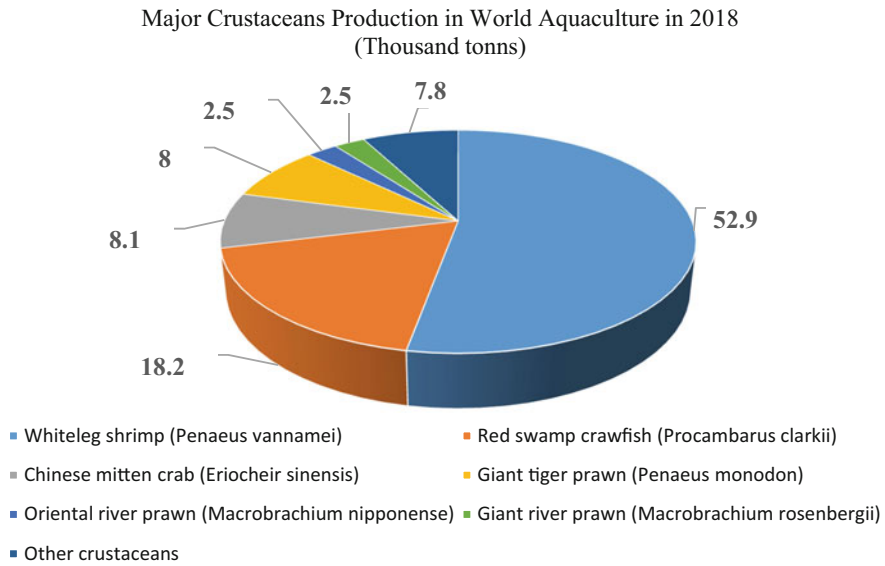
Fig. 1.1 Percentage of major crustaceans’ production in world aquaculture (FAO 2020)
