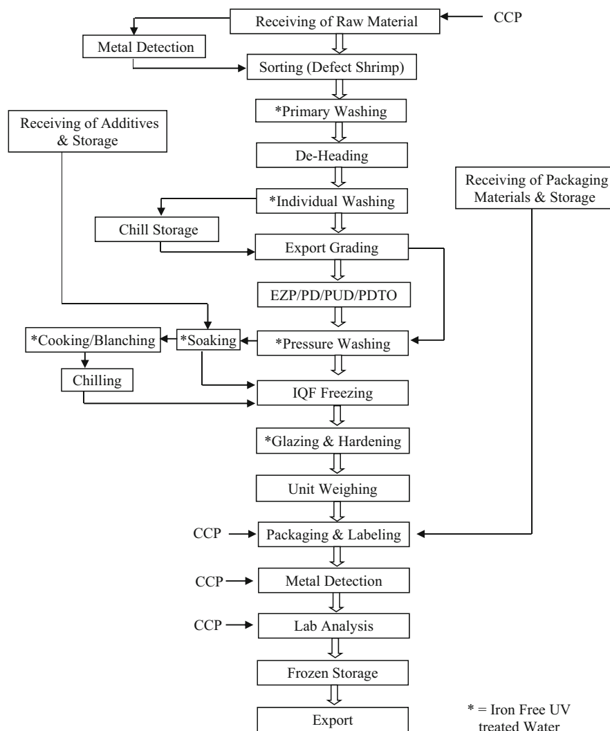
Fig. 2.25 Steps of IQF shrimp
